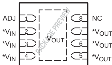
DRJ (QFN) PACKAGE (TOP VIEW)
